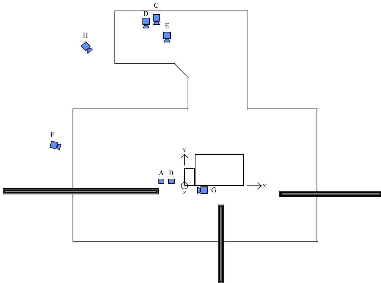
Figure 5 High-Speed Camera Positions
