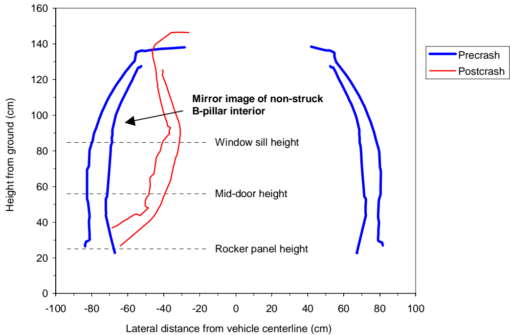
Figure 8 Example B-Pillar Vertical Profiles
