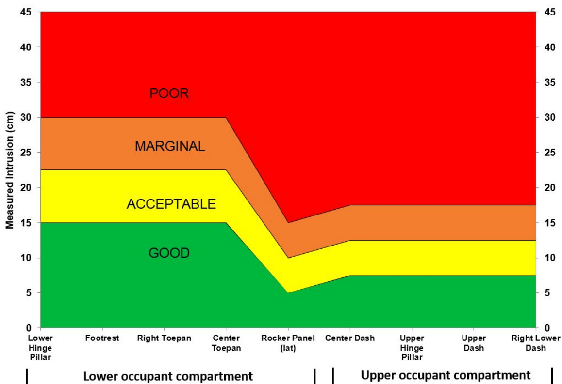
Figure A-7 Guidelines for Rating Front Passenger Occupant Compartment Intrusion
