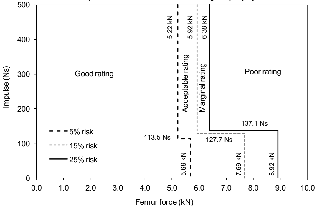
Figure 14 Force and Impulse Corridor Limits for Knee-Thigh-Hip Injury Risk
