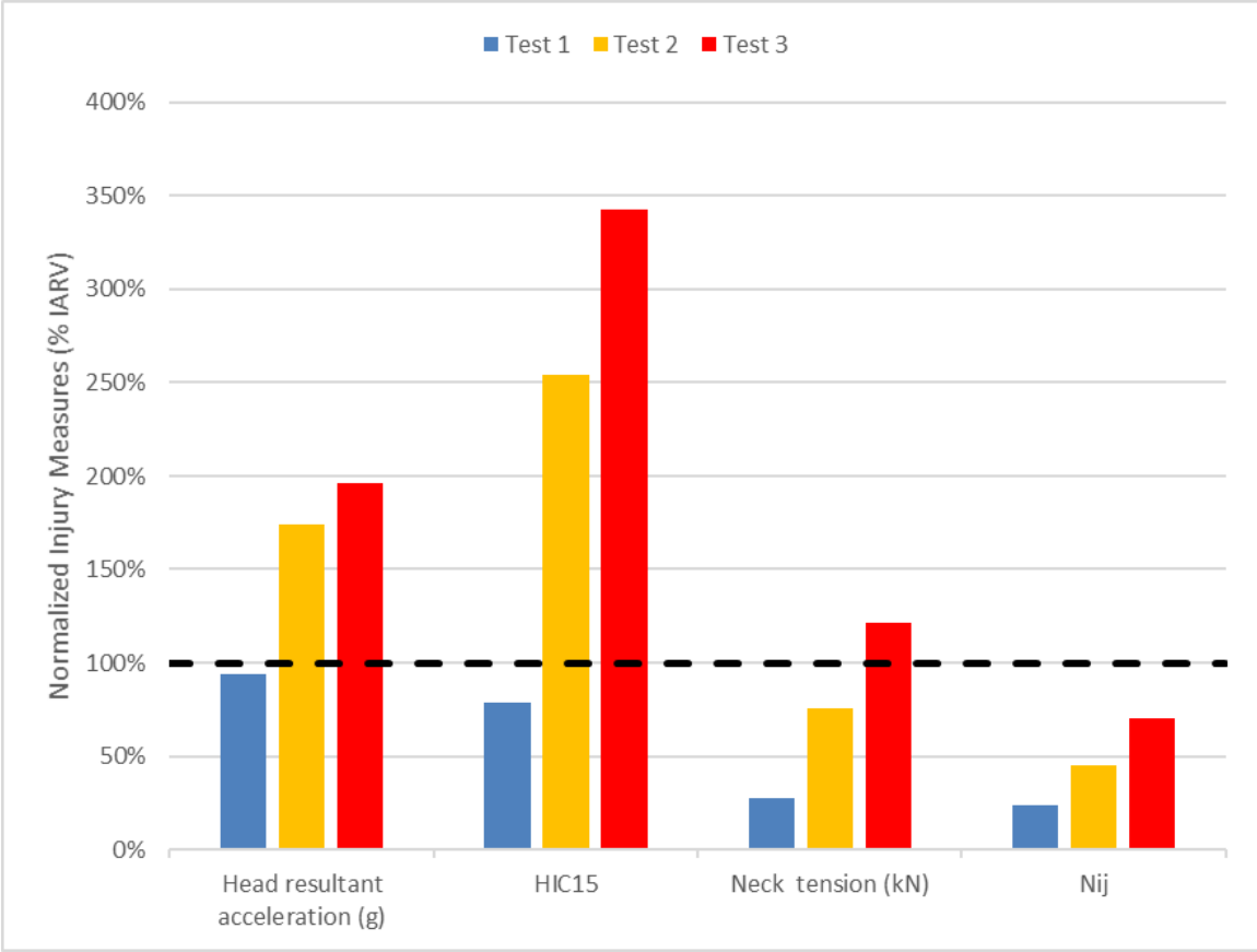
Figure 17. Head and neck injury measures normalized by IARV
