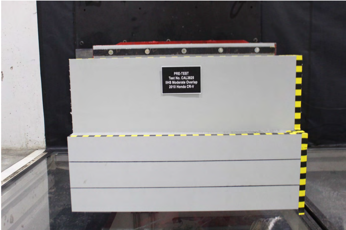
Figure 6. Side and front views of deformable barrier used for this study
