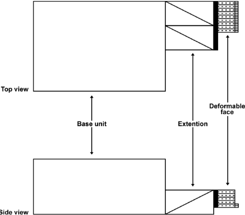
Figure 5. Deformable barrier composition Source: IIHS crash test protocol (IIHS, 2017)
